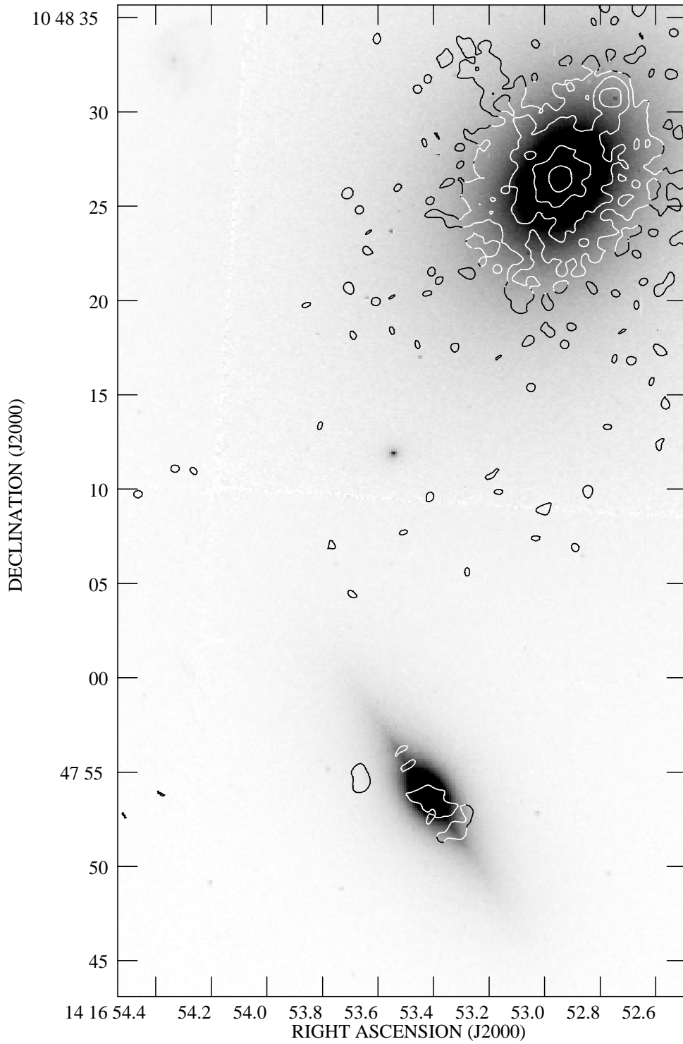
Figure 4. The X-ray emission detected by Chandra superposed on an archival Hubble Space Telescope WFPC2 image of the area around NGC 5532. The X-ray contours are from the smoothed X-ray image shown in Fig. 1; the lowest contour is at approximately 3\sigma above background (Hardcastle 2002). The HST image is the snapshot image in the F702W filter presented by Martel et al. (1999). The X-ray point source to the northwest of 3C 296 is close to a faint optical point source: the extended X-ray source to the south is associated with the spiral companion galaxy.
