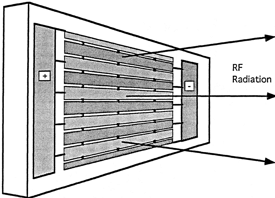
Figure 1. The figure illustrates an array with only 27 Josephson junctions. The array reported here has 638 junctions in it. However, the basic circuit idea is the same as shown in this figure.
